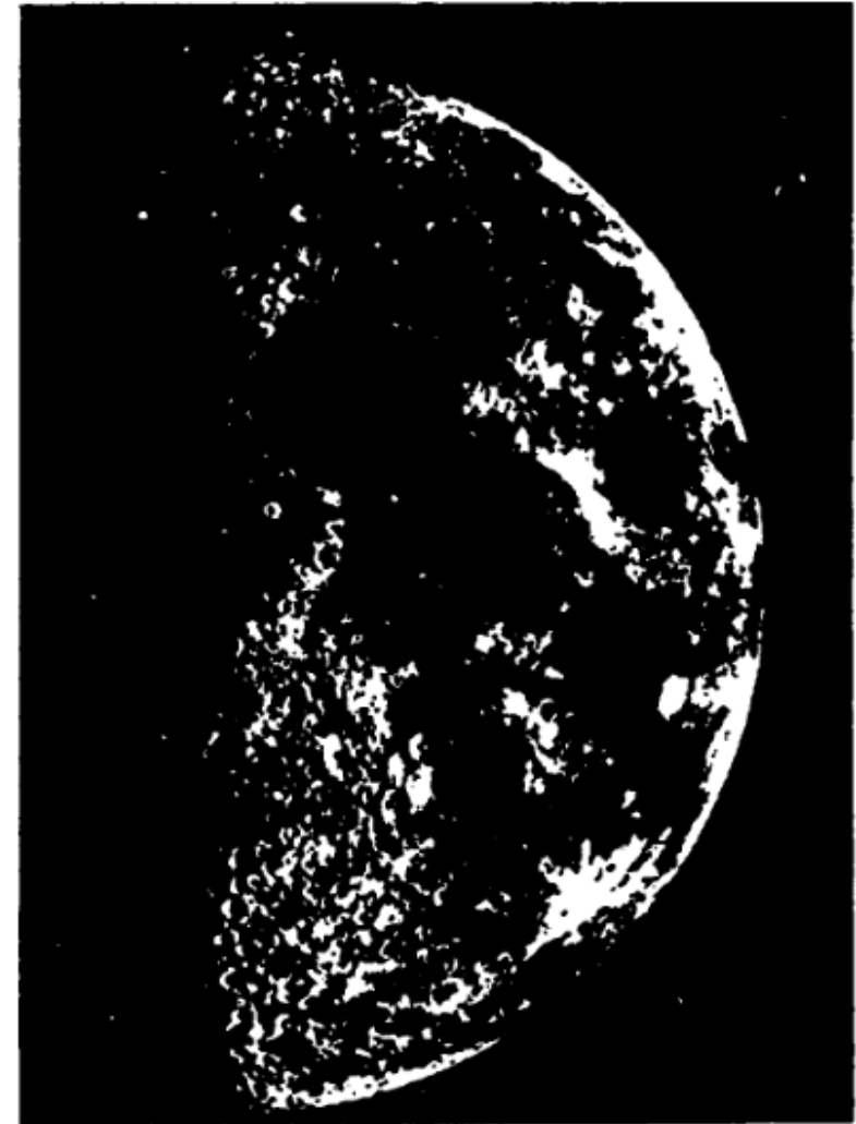
FIGURE 2. Moon, age seven days (first quarter).
